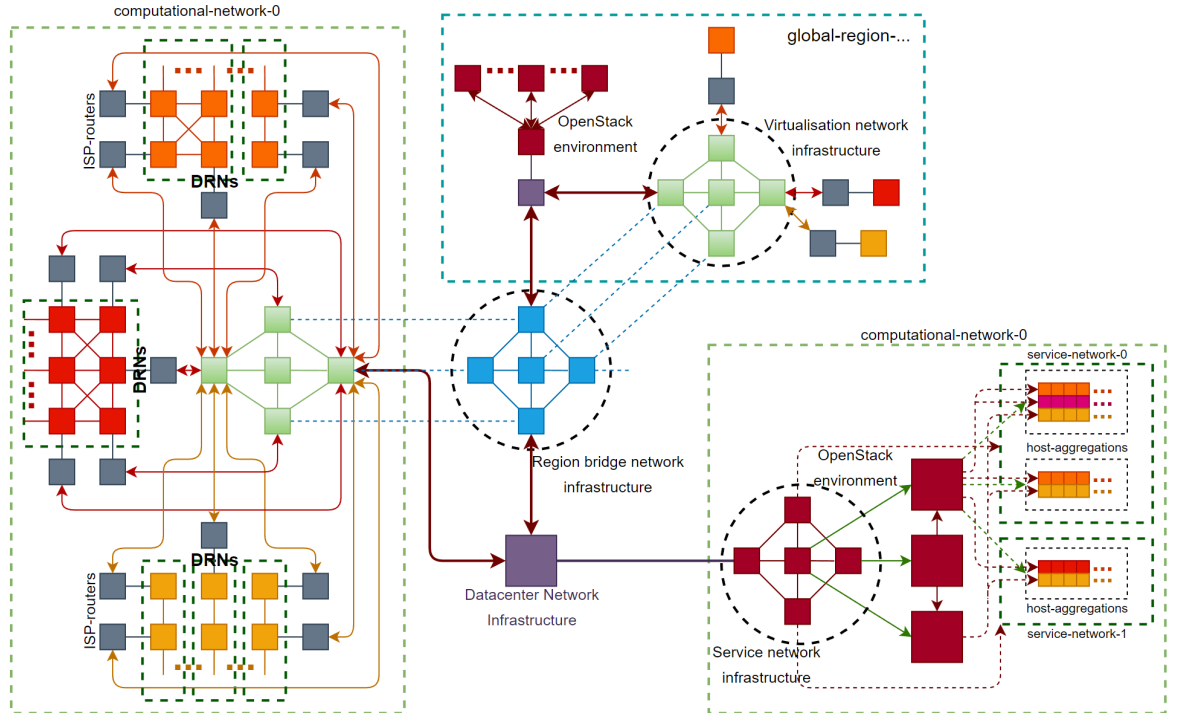
Figure 7: High-level overview of the DVCI Network approaches.
